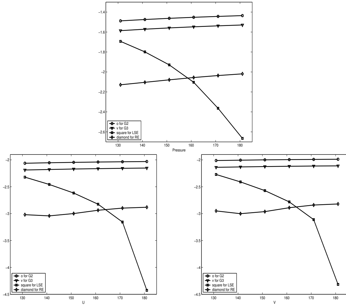
Fig. 5. Performance of LSE, with postprocessing of the residual, to predict the solution on the grid 181 \times 181 . The coarse grid solution G_1 , G_2 , G_3 , are respectively 101 \times 101 , 111 \times 111 , 121 \times 121 .
