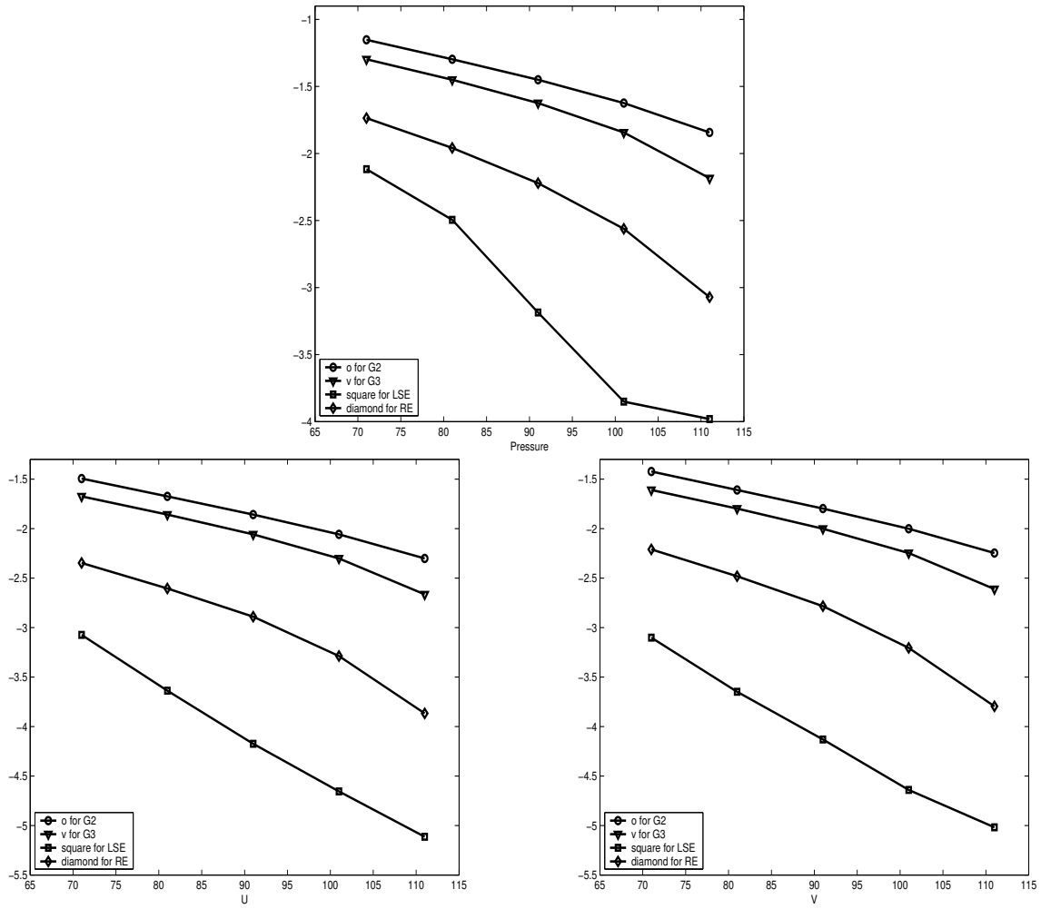
Fig. 6. Comparison of LSE versus RE with varying accuracy for the coarse grid solution. G_1 , G_2 , G_3 , are respectively (N - 20)^2 , (N - 10)^2 , N^2 grids. Horizontal axis gives the number of grid points N in each space direction for G_3 .
