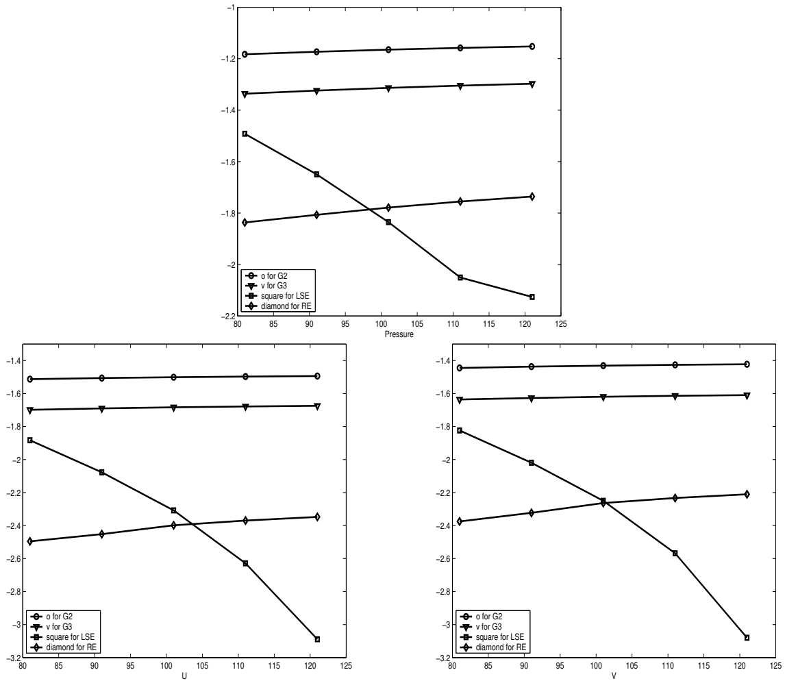
Fig. 4. Performance of LSE to predict the M^0 grid solution with the same notation and computation as in Figure 2 but with postprocessing of the coarse grid solution and the residual to filter out the high waves components.
