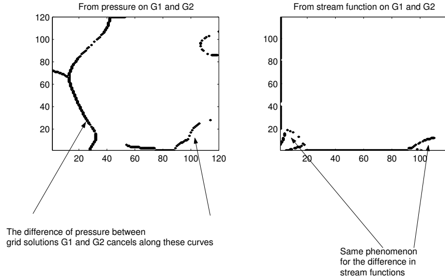
Fig. 1. Location of some local minima of \bar{p}_2 - \bar{p}_1 on the left and \tilde{\psi}_2 - \tilde{\psi}_1 on the right where cancellation with the two level's LSE take places.
