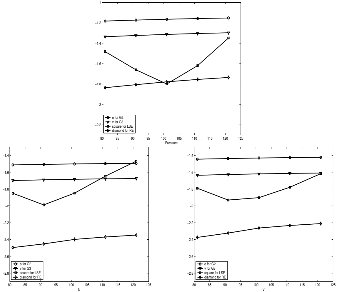
Fig. 3. Performance of LSE to predict the M^0 grid solution with the same notation and computation as in Figure 2.
