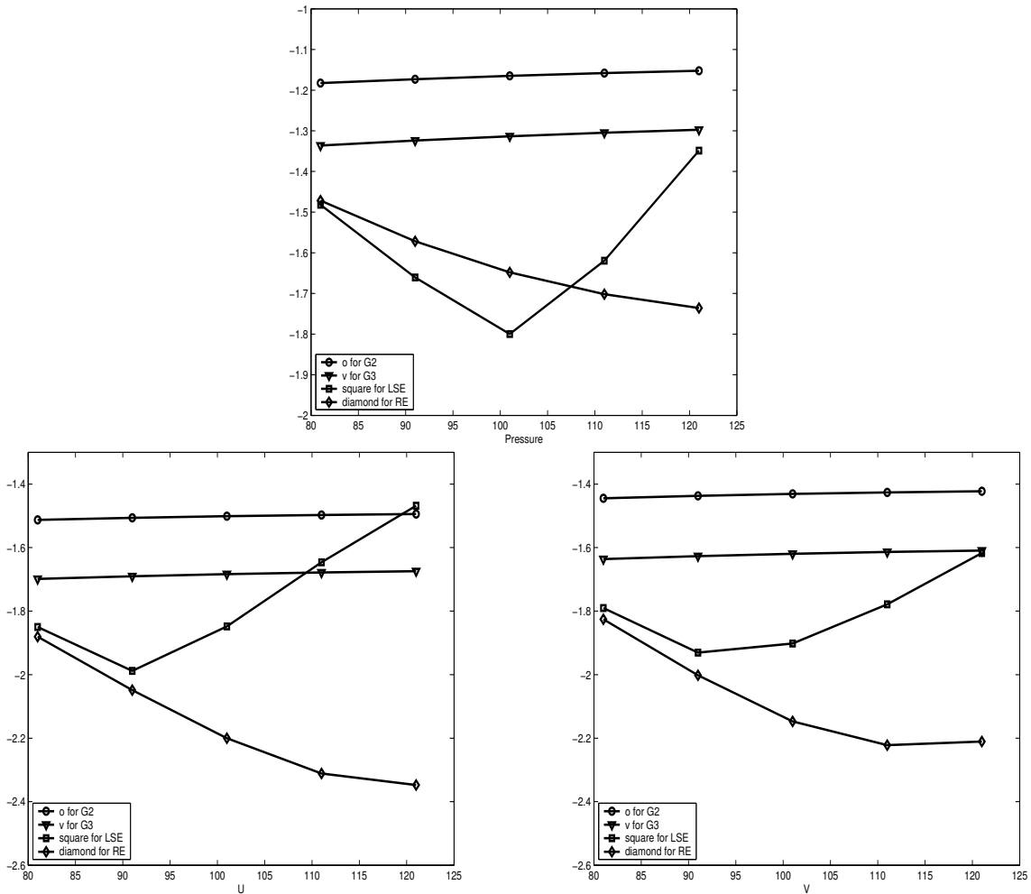
Fig. 2. Performance of LSE (without postprocessing of the residual) to predict the solution on the grid 121 \times 121 . The coarse grid solution G_1, G_2, G_3 , are respectively 51 \times 51, 61 \times 61, 71 \times 71 .
