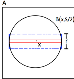
Figure 2.2: Illustration of the main idea of the proof of Proposition 2.2. As r \rightarrow 0 the parallelepiped [-\frac{s}{2}, \frac{s}{2}] \times [-\frac{r}{2}, \frac{r}{2}] is almost contained in B(x, s/2) if x is a point of isotropy of A at scale s , forcing \mathcal{D}_{s,r}\chi_A(x) = 1 as r goes to 0.
