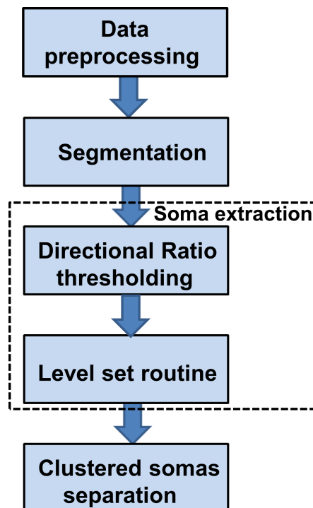
Figure 3.1: Proposed algorithm for 2D soma detection.
