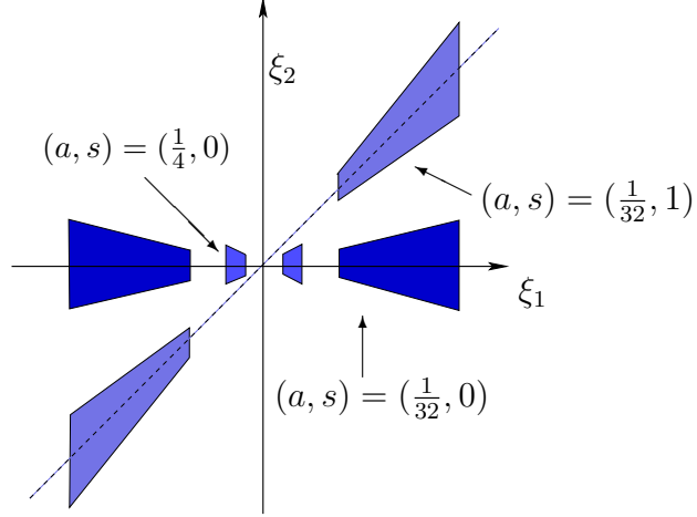
Figure 1.1: Frequency supports of the horizontal shearlets \hat{\psi}_{a,s,t}^{(h)} for different values of a and s .
