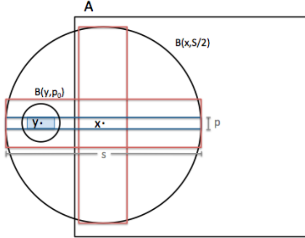
Figure 2.4: Illustration of the main idea of the proof of Proposition 2.4
