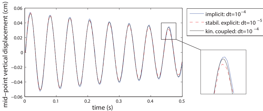
Figure 3: Mid-point vertical displacement computed using a monolithic scheme (blue solid line) with \Delta t = 10^{-4} , a stabilized explicit scheme proposed by Burman and Fernandez [17] with \Delta t = 10^{-5} (red dashed line), and the operator splitting scheme with \beta = 1 and \Delta t = 10^{-4} (black solid line).
