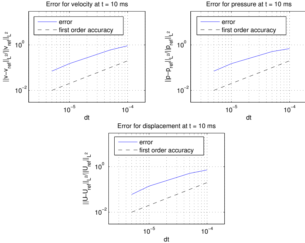
Figure 10: Example 1: Figures show relative errors obtained at t=10 ms. Top left: Relative error for fluid velocity. Top right: Relative error for fluid pressure. Bottom: Relative error for the structure displacement.
