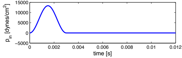
Figure 4: The inlet pressure pulse for Example 2. The outlet normal stress is kept at 0.
