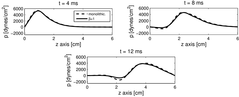
Figure 8: Mean pressure vs. z , at t = 4, 8, 12 ms, computed with the monolithic scheme by Quaini [66] (time step \Delta t = 10^{-4} ; dashed red line), and with our operator splitting scheme with \beta = 1 (time step \Delta t = 5 \times 10^{-5} ; solid blue line).
