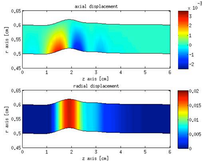
Figure 6: The longitudinal (top) and radial (bottom) components of the structure displacement. Notice how the red and blue colors in longitudinal displacement denote longitudinal stretching of the structure in opposite (+/-) directions.
