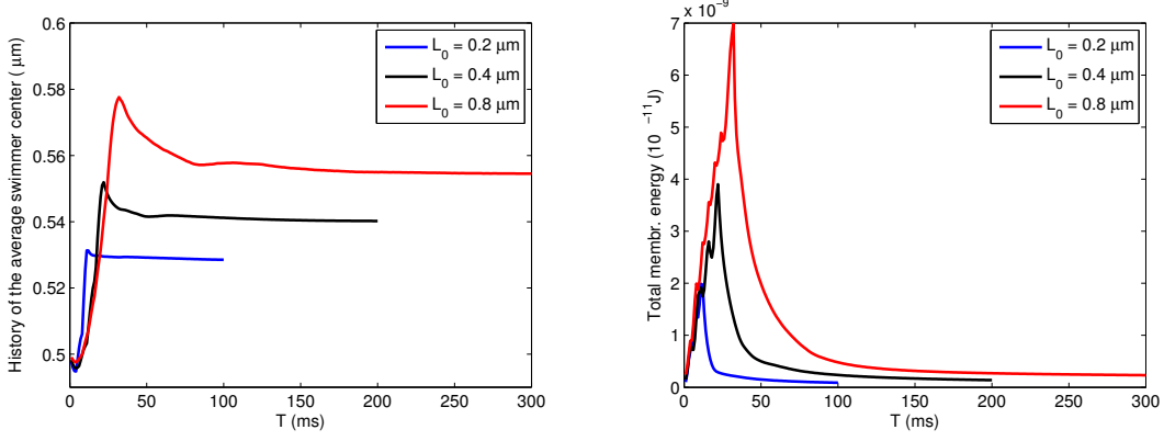
Figure 6: History of motion of swimmer center (left) and of total energy (right) for the three swimmers shown in Figure 5.
