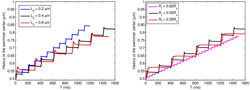
Figure 14: The figures show history of swimmers center for multiple cycles of force application. Left: comparison between swimmers of different reference length, same reference radius R_0 = 0.125\mu m , and same deformed radius R_f = 0.55R_0 , c.f. Figure 6. Right: comparison between swimmers with different deformed radius, same reference radius R_0 = 0.125\mu m and same reference length L = 0.4\mu m , c.f. Figure 8.
