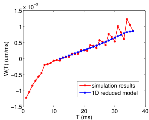
Figure 11: A comparison between swimmer velocity obtained using full 3D simulations (red) and the reduced 1D model (54) (blue). We see excellent agreement between the two in the regime where the swimmer velocity is positive.
