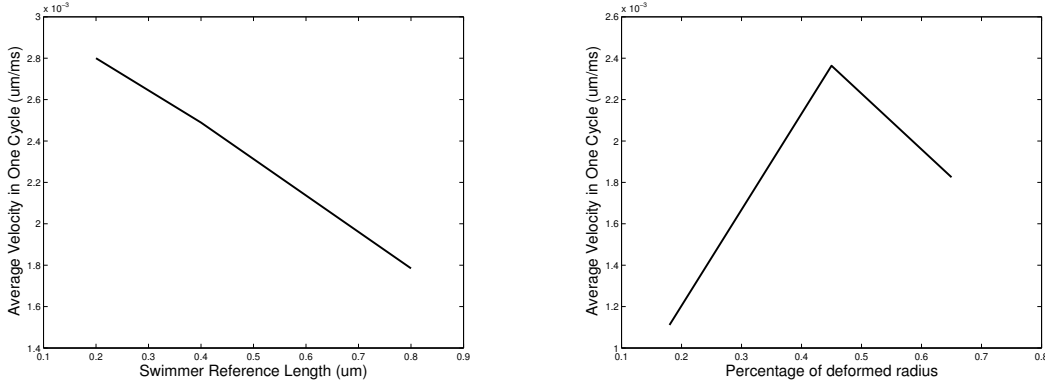
Figure 13: Average velocity of swimmers during one cycle of force application. Left: Swimmers with different lengths ( L = 0.2, 0.4, 0.8\mu m ) and same reference radius R_0 = 0.125\mu m . Right: Swimmers with same reference length ( L = 0.4\mu m ) and radius ( R_0 = 0.125\mu m ) but different traveling wave amplitude (percentage of deformed radius 0.18%, 0.45%, 0.65%).
